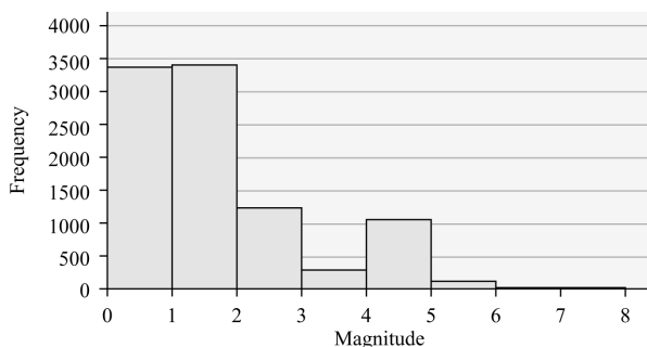
Magnitude of Earthquakes Worldwide: October 2014
